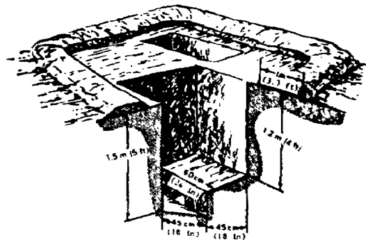
Figure 1-20. Two one-man foxhole type machinegun emplacement.
